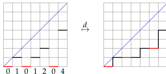
Figure 2: The outline of inversion sequence (0, 1, 0, 1, 2, 0, 4) .
